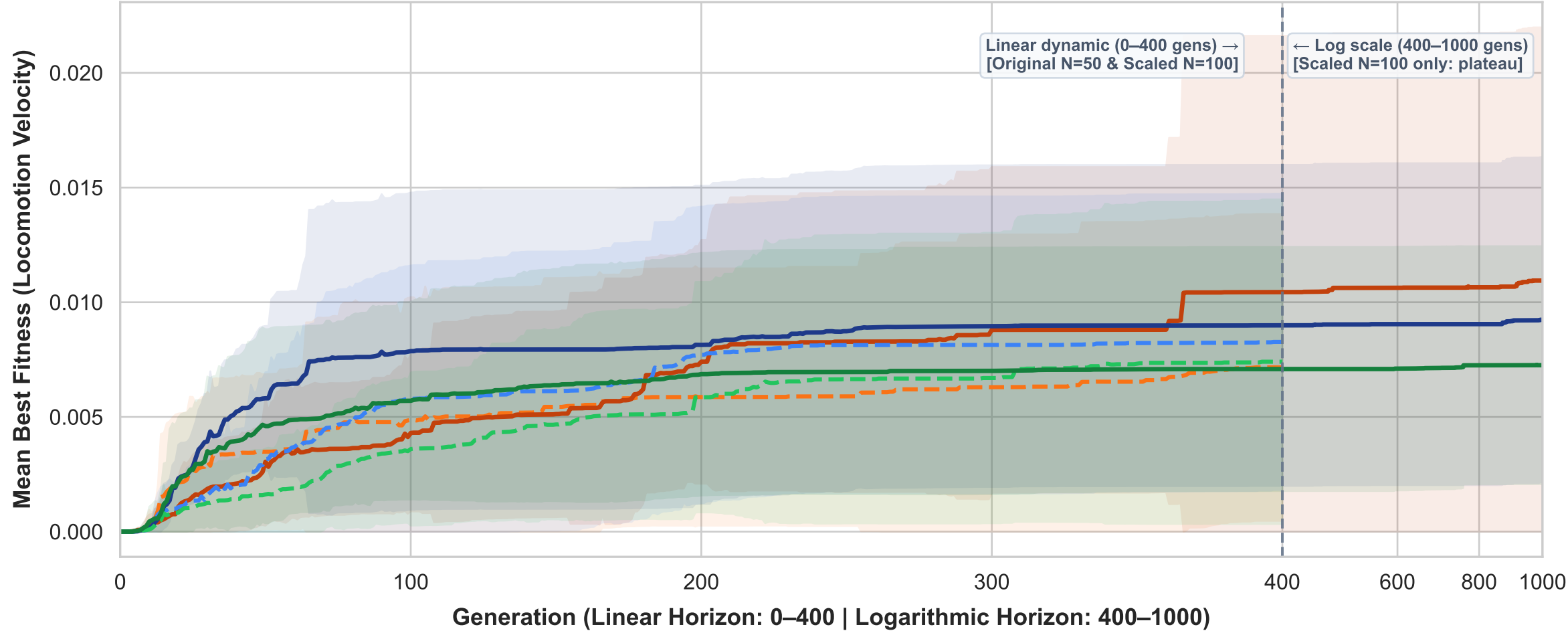
Mean Best Fitness & Confidence Intervals ( mean \pm 1\sigma ): Lin-Log Generational Dynamic Original ( N = 50 , dashed) vs. Scaled ( N = 100 , solid) Champions Across 10 Replications
